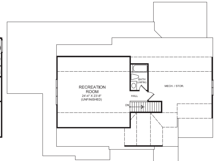
THIRD FLOOR
